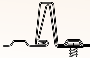
HIDDEN FASTENER PANEL CANADIAN PATENT: # 1259466 USA PATENT: # 4926608
