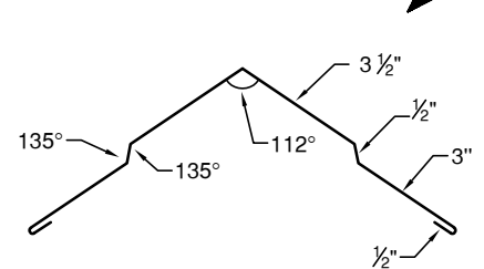
LIBERTY RIDGE CAP (15" GIRTH)
