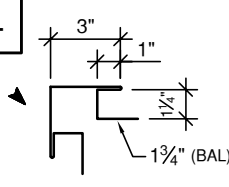
COMMERCIAL OUTSIDE CORNER (14" GIRTH)
