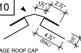
COTTAGE ROOF CAP FOR COMMERCIAL RIB PROFILE (24" GIRTH)
