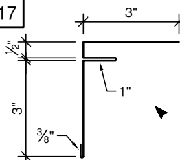
SIDING / SOFFIT "F-J" TRIM (8 3/8" GIRTH, 26g)
