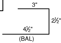
"J" CLOSURE (10" GIRTH, 24G, GALVANIZED)
