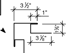
OUTSIDE CORNER (18" GIRTH)
