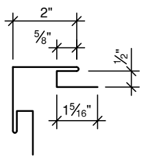
OUTSIDE CORNER (8 3/8" GIRTH, 26g)
