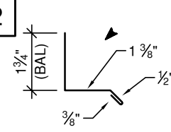
COMMERCIAL BASE FLASHING (4" GIRTH)
