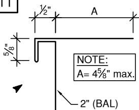
WINDOW & DOOR JAMB (4 1/4" + A = GIRTH (8 3/8" max.), 26g)
