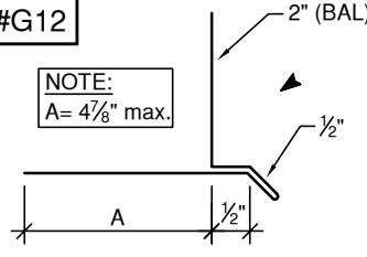
WINDOW & DOOR FLASHING (4" + A = GIRTH (8 3/8" max.), 26g)
