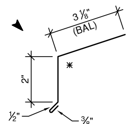
STEEL ROOFING DRIP EDGE (6" GIRTH) * SPECIFY PITCH
