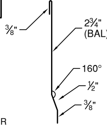
STARTER (4" GIRTH, 26g, GALVANIZED)
