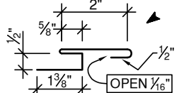
WINDOW & DOOR FLASHING (4" + A = GIRTH (8 3/8" max.), 26g)
