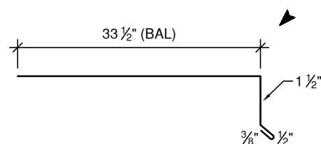
ICE APRON (for shingles) (36" GIRTH)
