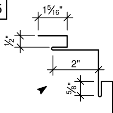
INSIDE CORNER (8 3/8" GIRTH, 26g)
