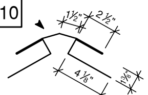
COTTAGE ROOF CAP (24" GIRTH)
