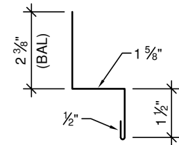
INDUSTRIAL GABLE DIVIDER (6" GIRTH)
