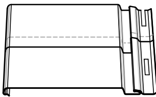
OVERLAP DETAIL
